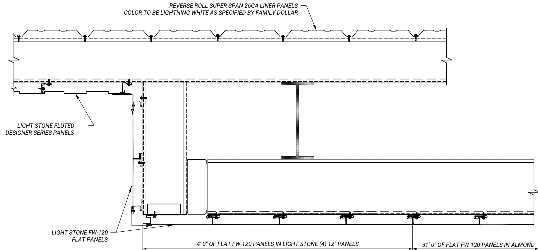
SECTION "B" ABOVE STOREFRONT
