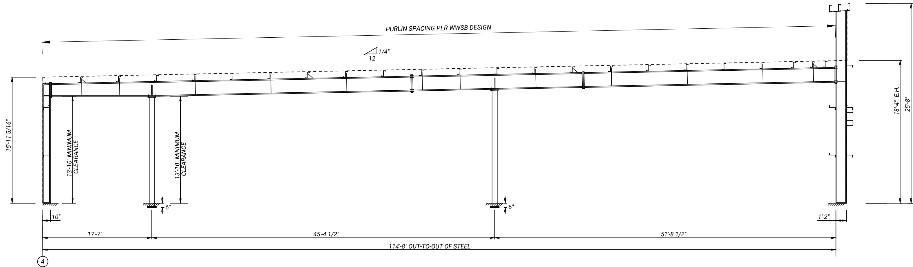
FRAME CROSS SECTION: FRAME LINE B & C
