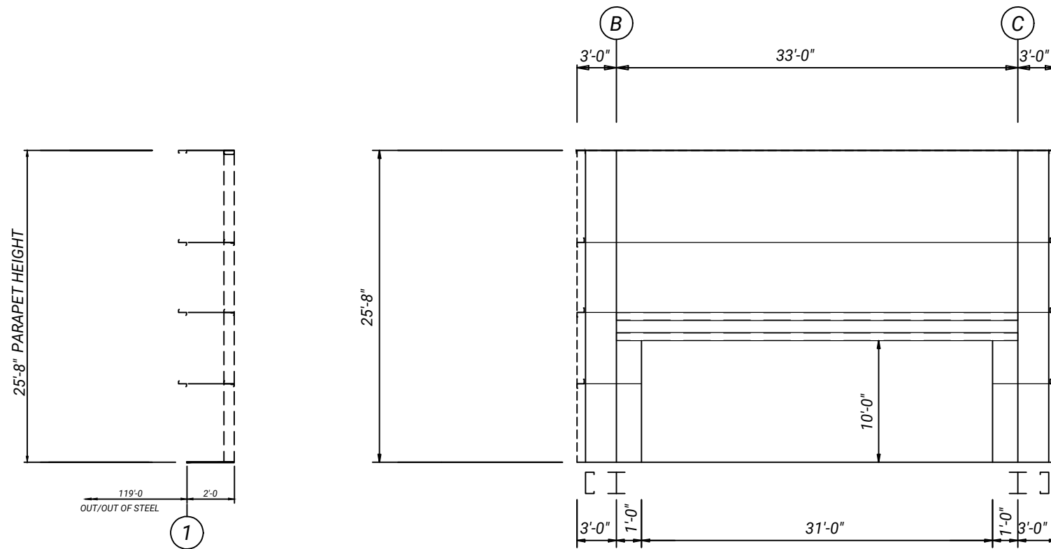
PARAPET ELEVATION FRAME LINE "B"
