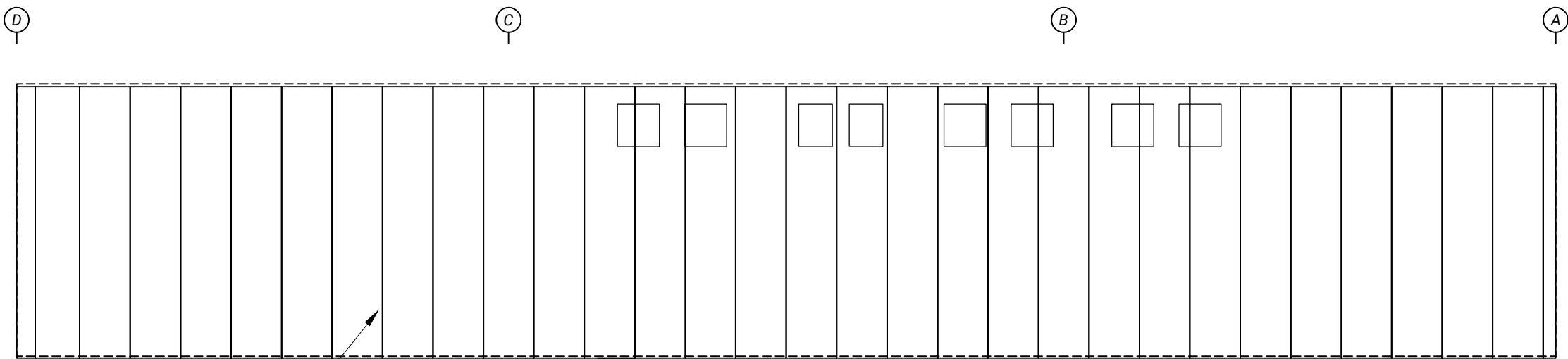
SIDEWALL FRAMING: FRAME LINE 4
