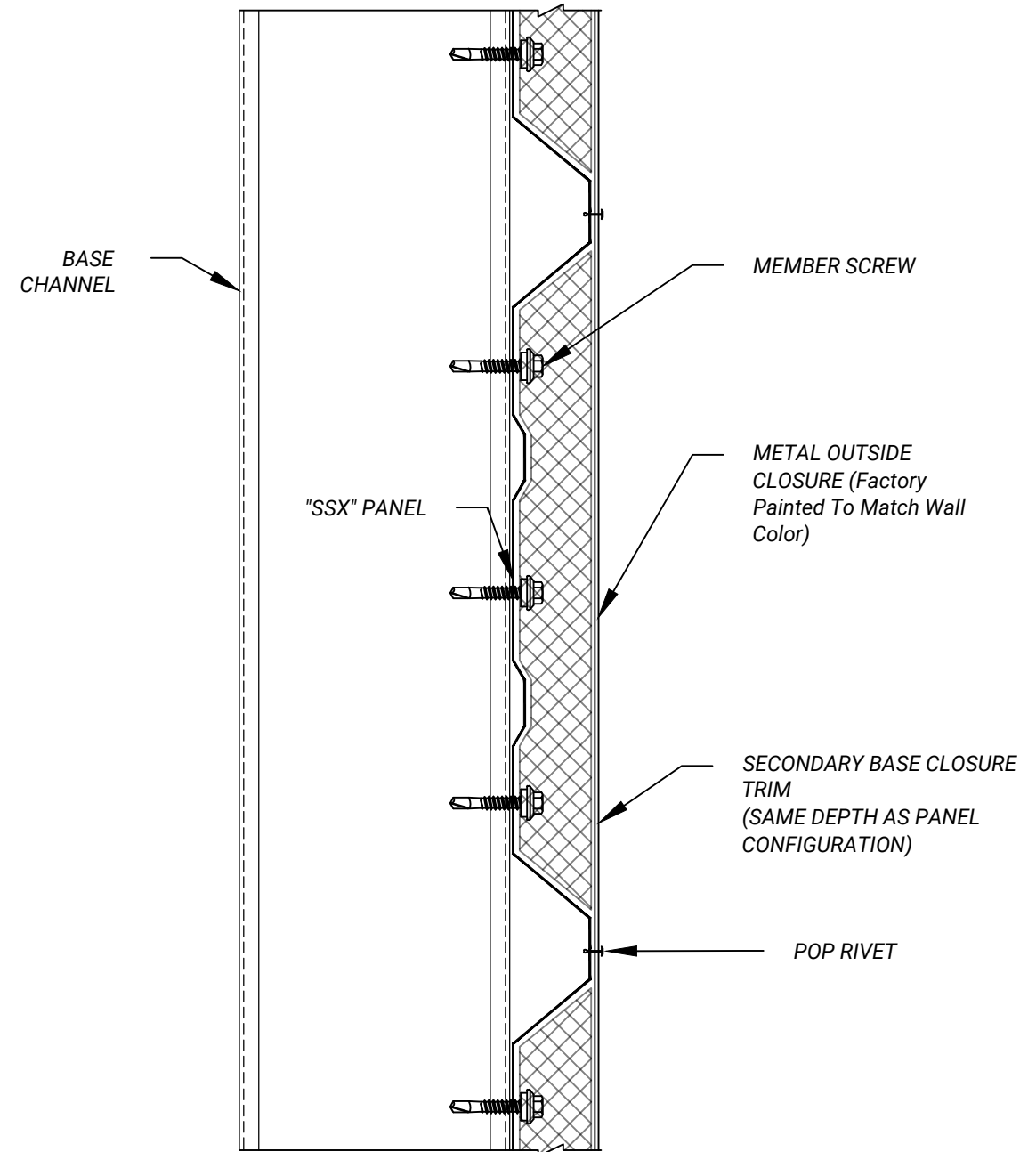
SECTION "A"
