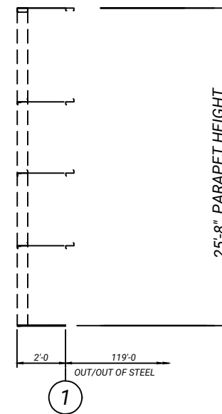
PARAPET ELEVATION LINE "C"
