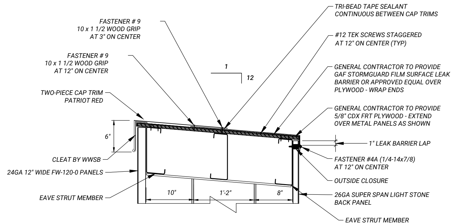
SECTION 'M'
