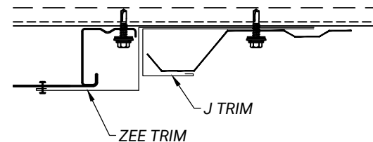
TRANSITION BETWEEN DESIGNER SERIES AND SUPER SPAN PANELS AT GRID LINES A & D
