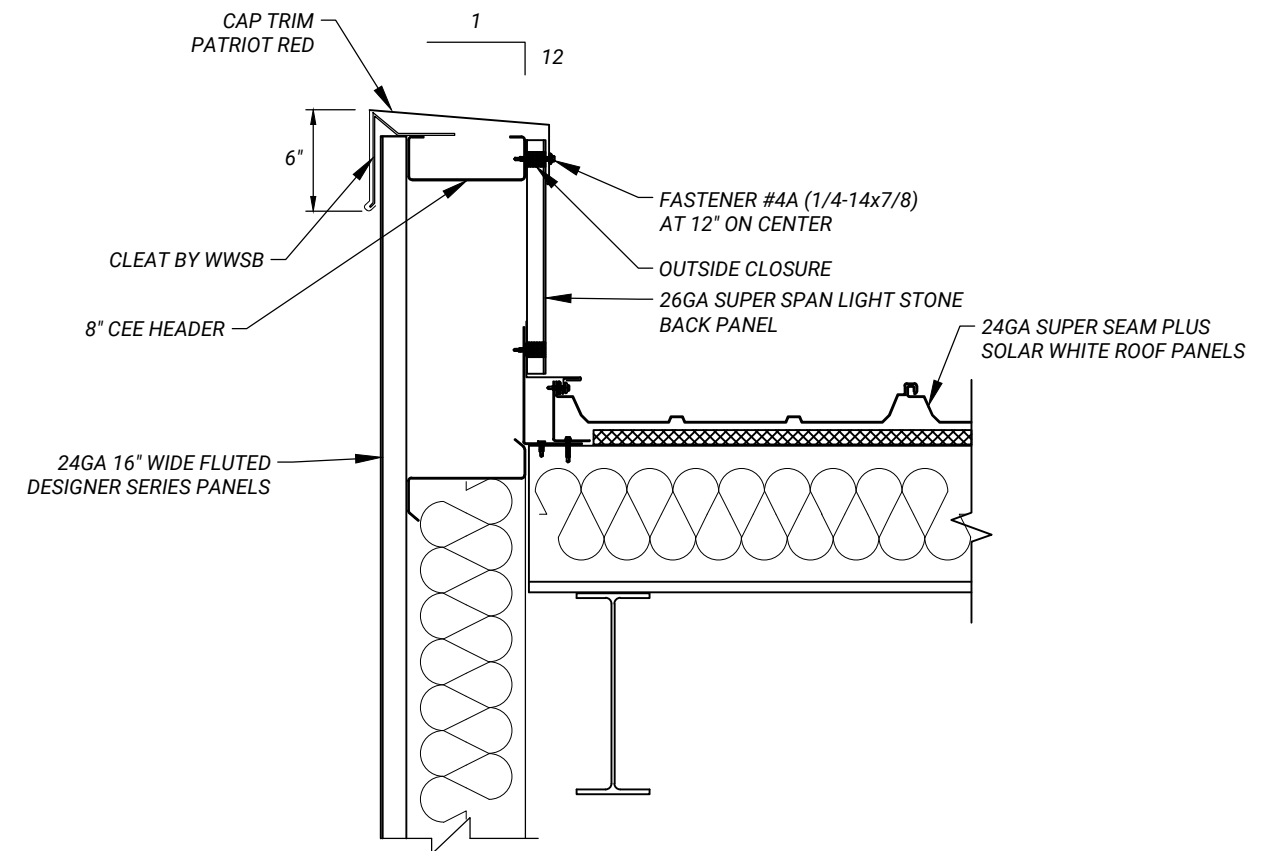
SECTION 'P'
