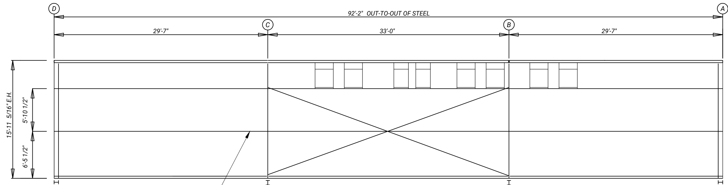
SIDEWALL FRAMING: FRAME LINE 4
