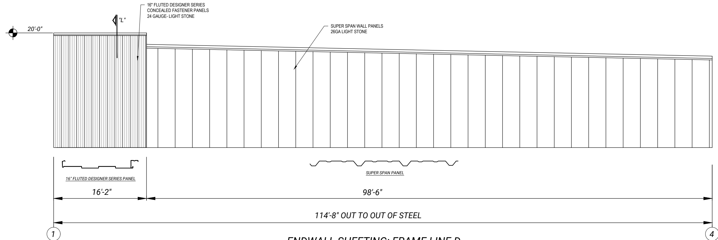
ENDWALL SHEETING: FRAME LINE D
