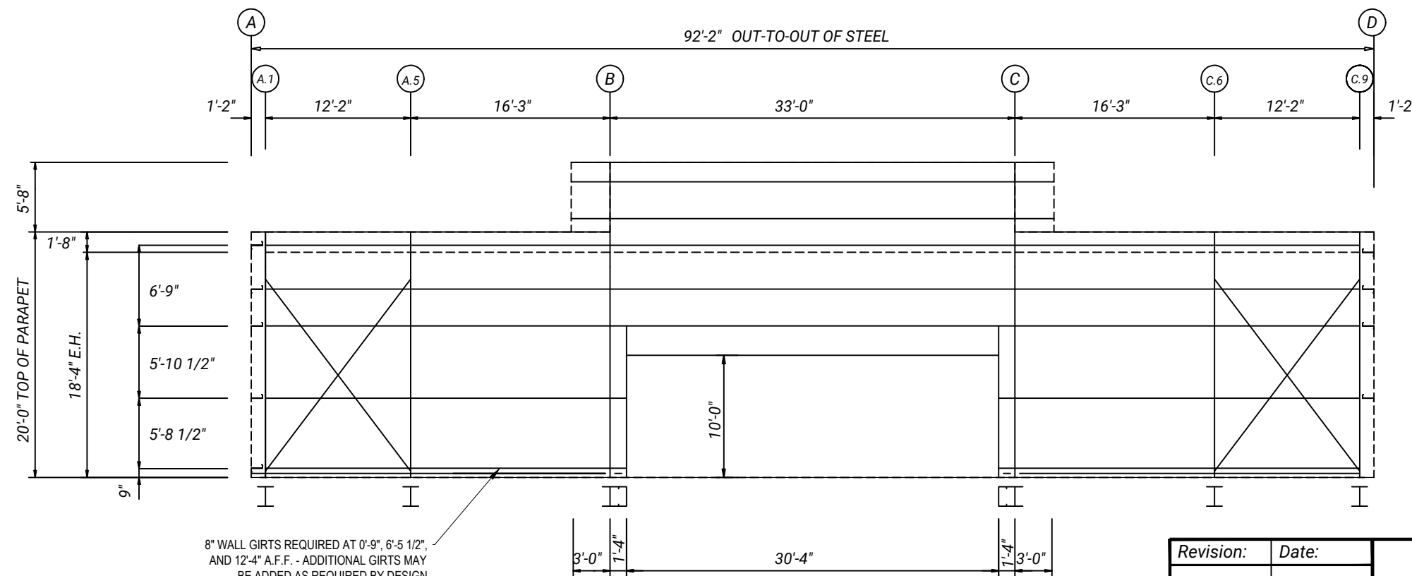
SIDEWALL FRAMING: FRAME LINE 1
