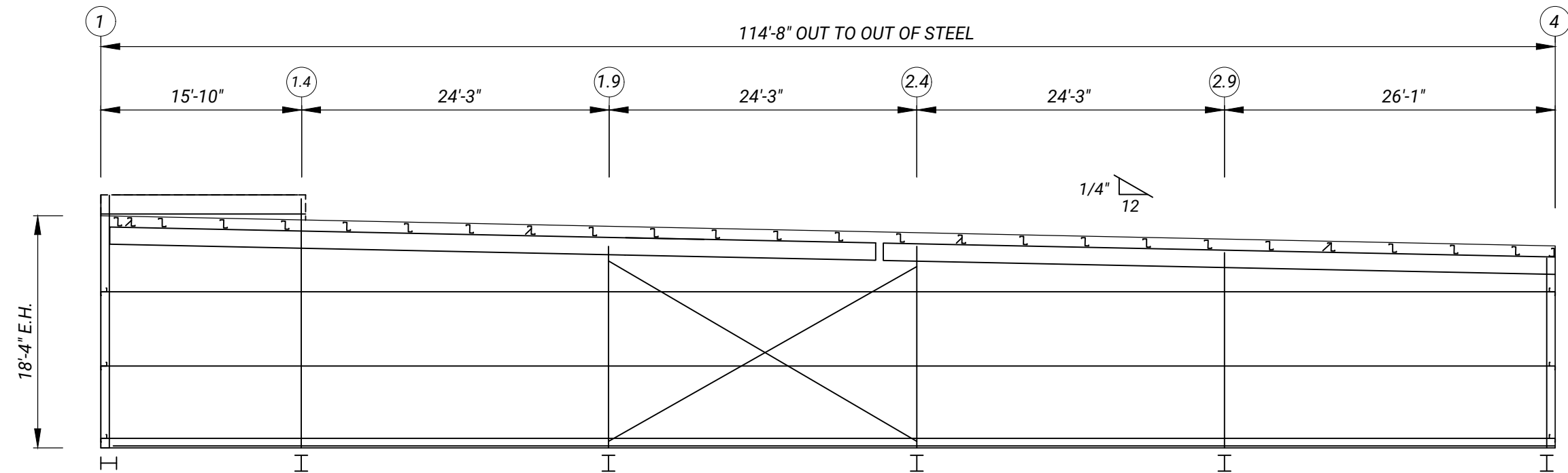
ENDWALL FRAMING: FRAME LINE D
