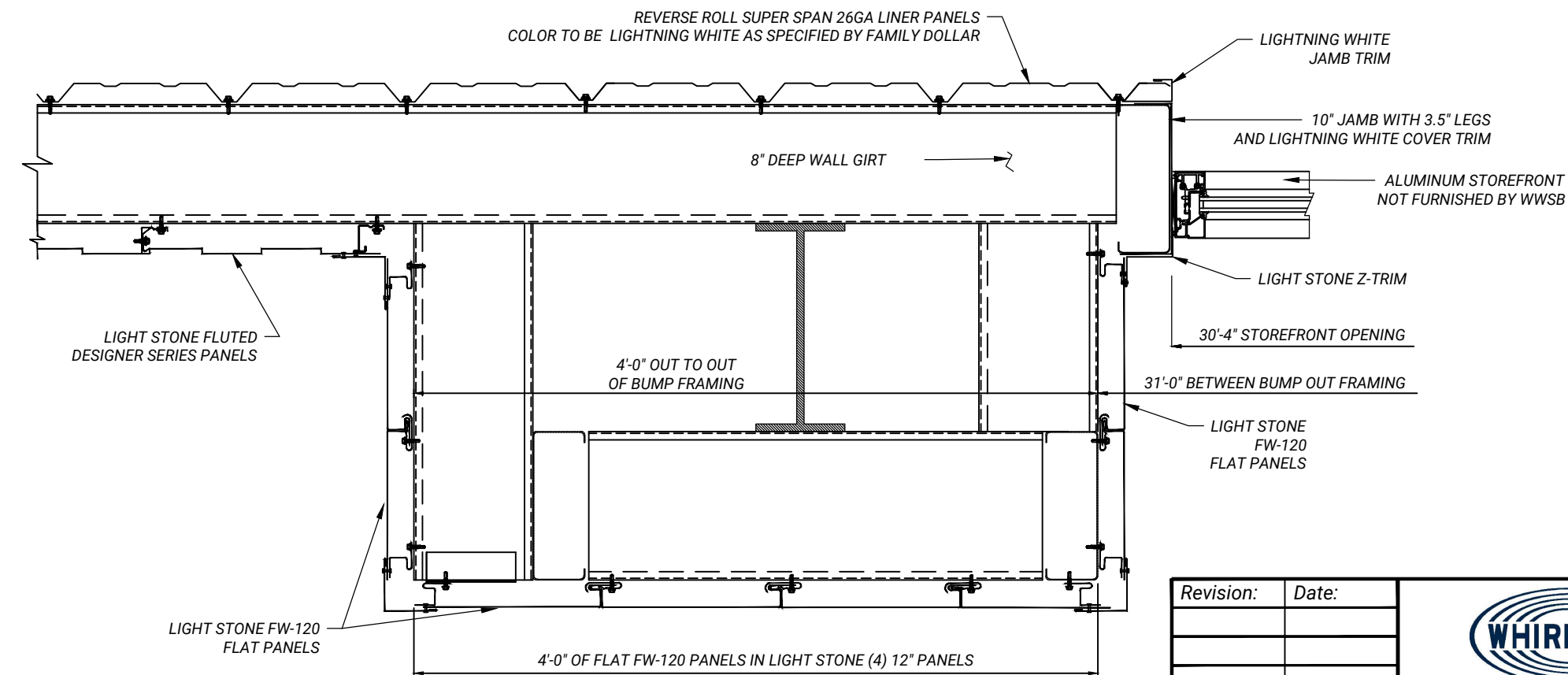
SECTION "C" BELOW 10' ELEVATION
